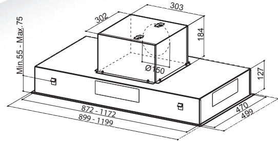
Air outlet adjustable in 4 positions
